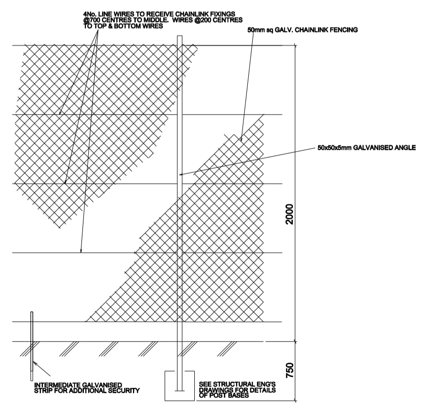
FENCE TYPE 2 - CHAIN LINK FENCE DO NOT SCALE USED AROUND CAR PARK AREA
